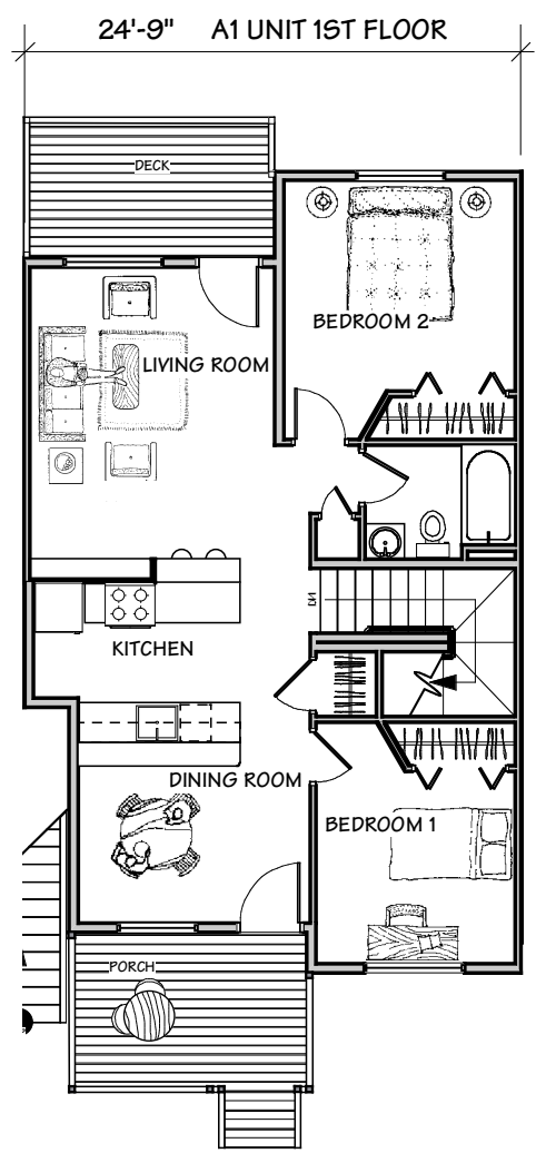
1 A1 UNIT PLANS @ 3/32"=1'-0" : SECTION @ 1/16"=1'-0"
