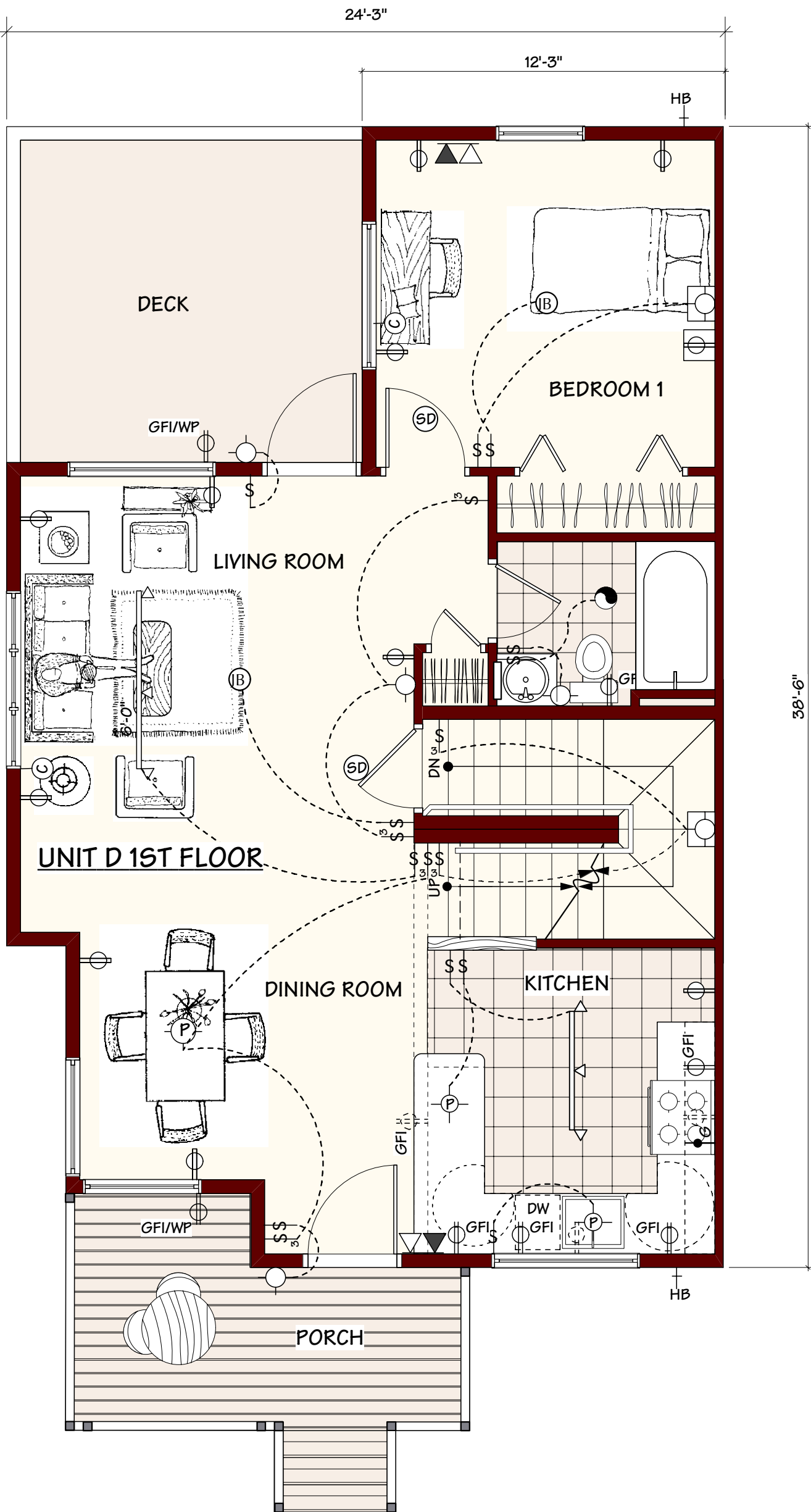
1 D UNIT FIRST FLOOR Scale: 1/4"=1'-0" D UNIT: 1375 SQ FT FINISHED 3bd/2.5ba 200-900 SQ FT UNFINISHED *square footages given are approximate
